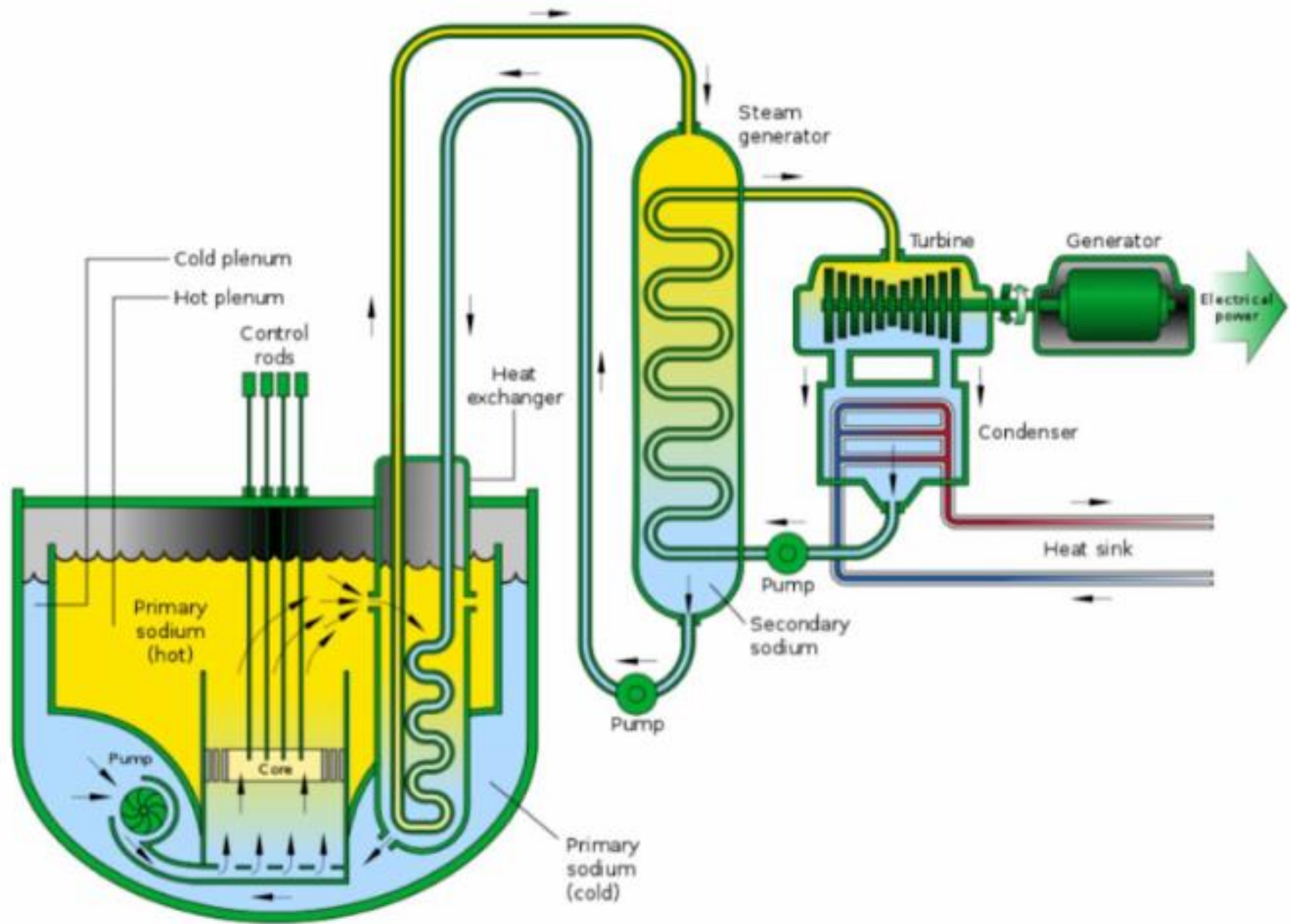
Pool type sodium-cooled fast reactor (SFR)
